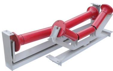
Friction self-aligning carrying and return idler/roller set
