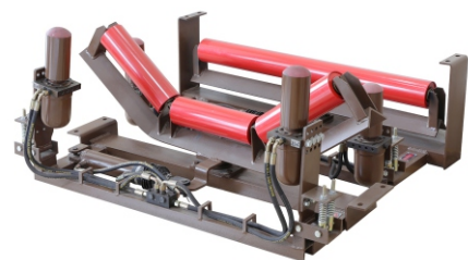
Hydraulic edge-correcting idler/roller set
